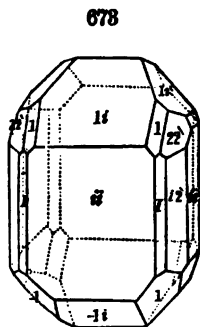
Watertown, Ct.
